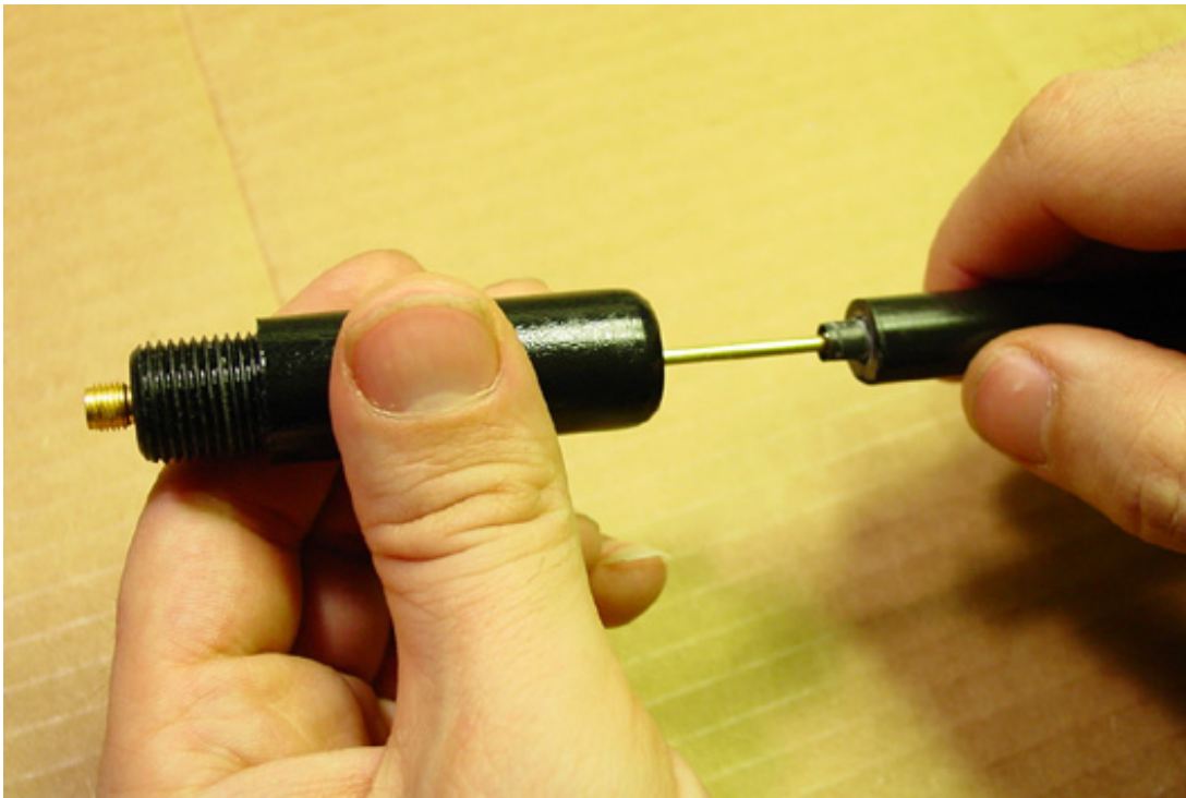
Figure 16. Retracting the radome once decoupler is set.
