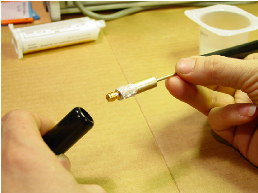
Figure 14. Epoxy applied to decoupler and about to be aligned into the threaded mounting component.
