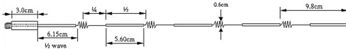
Figure 4. Antenna segment measurements.
